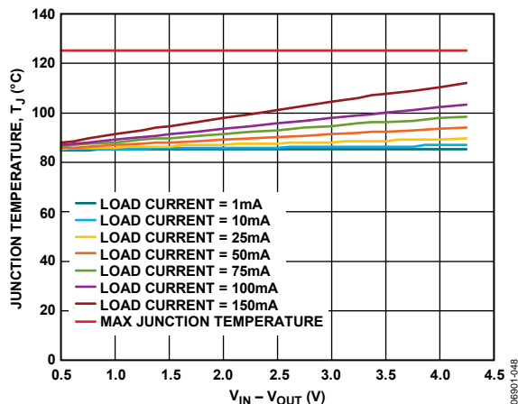
Figure 46. TSOT, 100 mm 2 of PCB Copper, T A = 85°C
