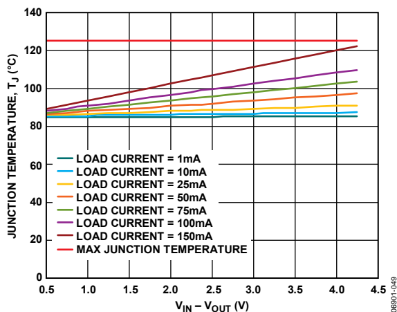
Figure 47. WLCSP, 100 mm 2 of PCB Copper, T A = 85°C
