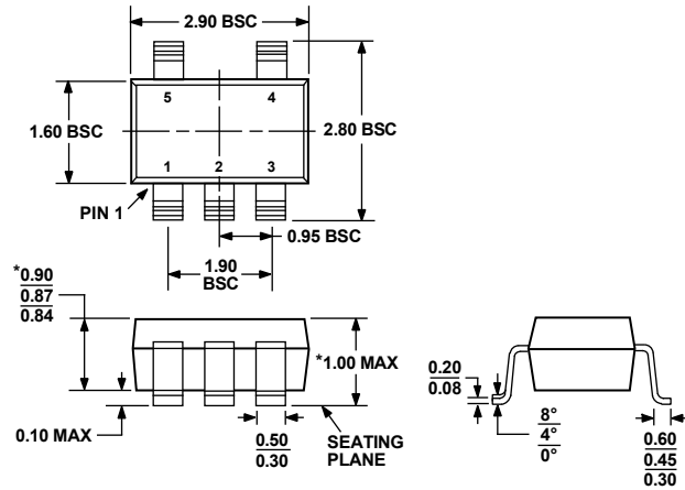
Figure 50. 5-Lead Thin Small Outline Transistor Package [TSOT] (UJ-5) Dimensions show in millimeters
